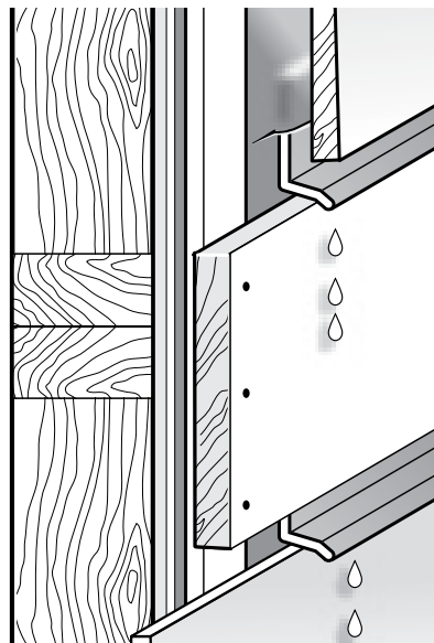
Second Story Bandboard
